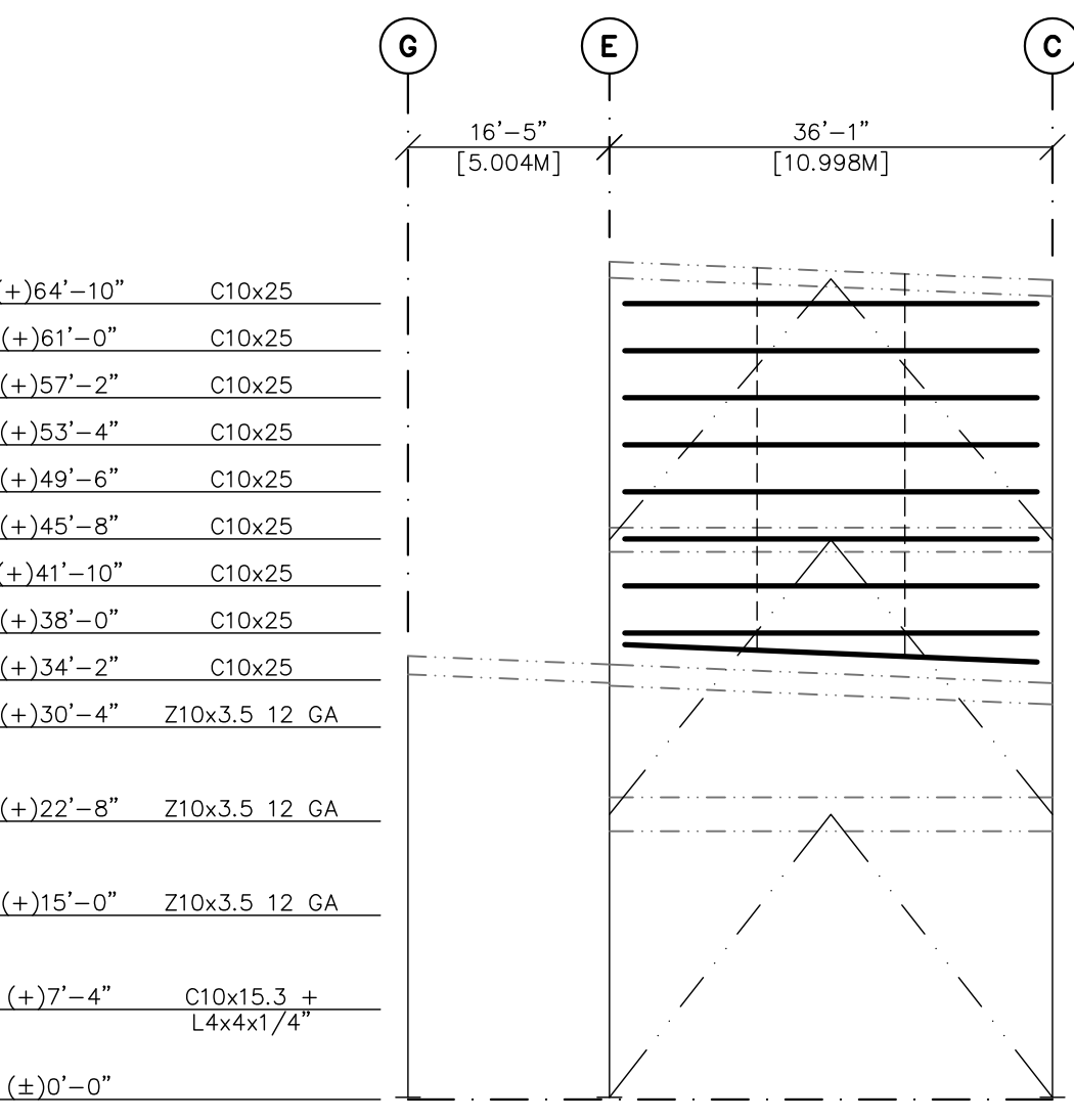
PARTIAL ELEVATION @ 3 LINE
