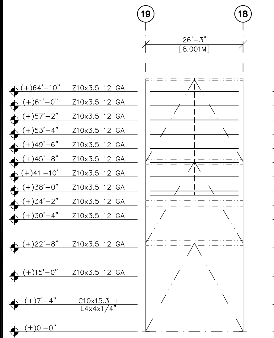
PARTIAL ELEVATION @ K LINE
